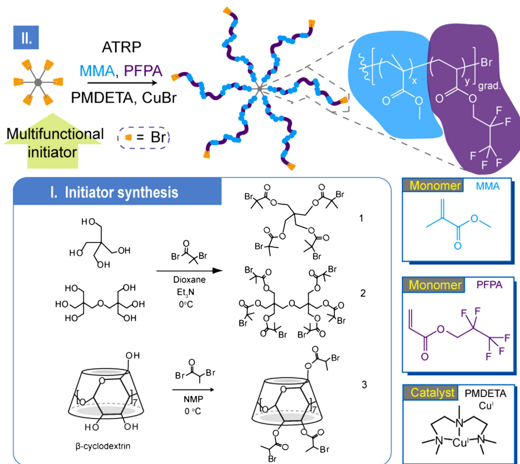
Scheme 1. Synthesis of (i) multifunctional initiators 1 , 2 , and 3 , and (ii) fluorinated star polymers with varying PFPFA monomer content using the multifunctional initiators via the core-first approach and ATRP. The PFPFA monomer content was controlled by varying the ratio of methyl methacrylate (MMA) to pentafluoropropyl acrylate (PFPFA).
